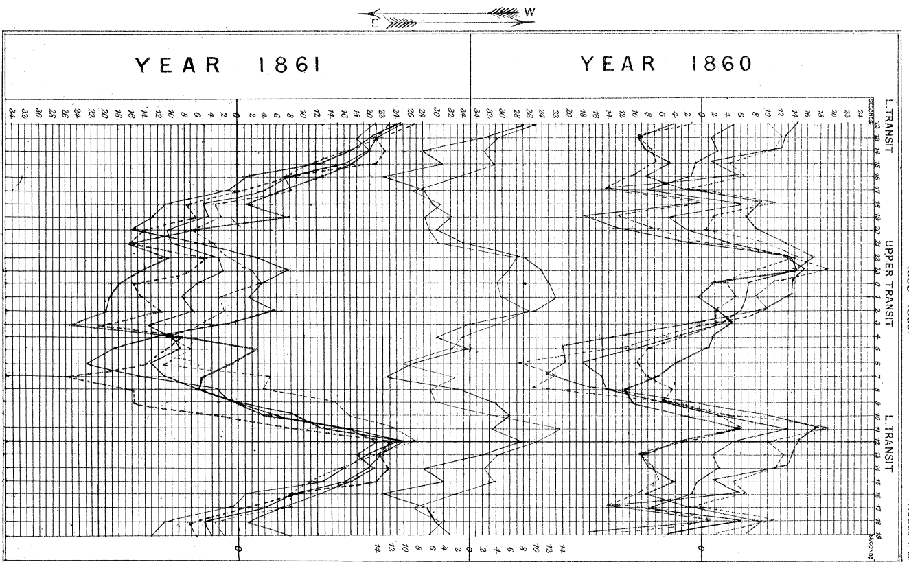
CURVES SHEWING THE LUNAR DIURNAL VARIATION OF THE MAGNETIC DECLINATION 1858-1863. TABLES II & III.
